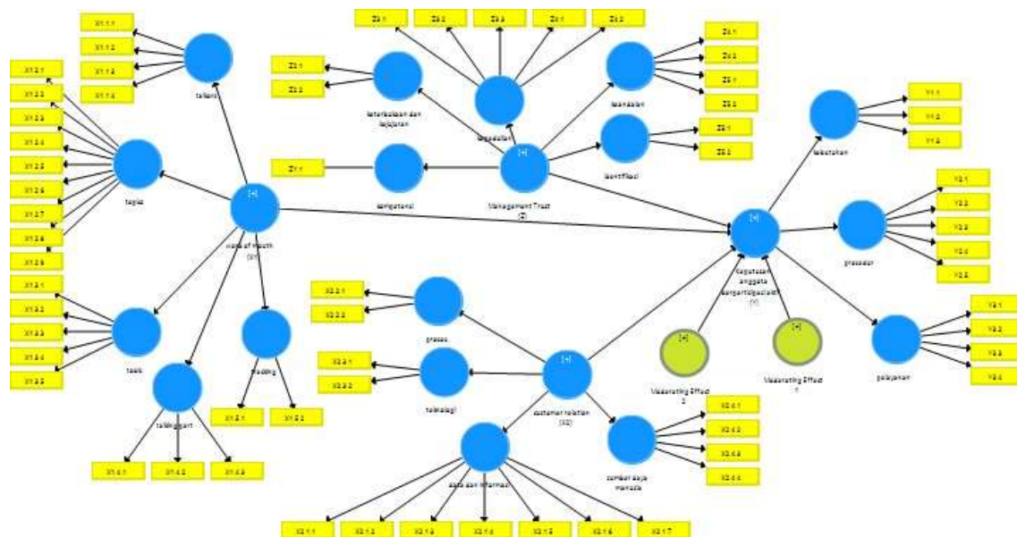
Gambar 2 Hasil Boostrapping
